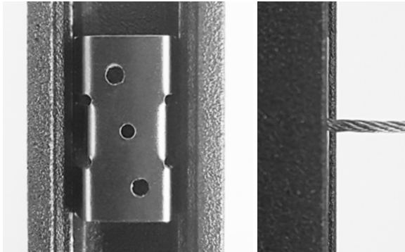
Correct Assembly.
