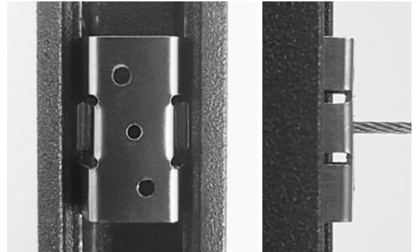
Incorrect Assembly.
